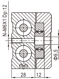
Across A-A
